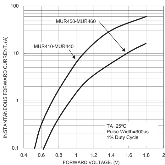
FIG. 5-TYPICAL FORWARD CHARACTERISTICS
